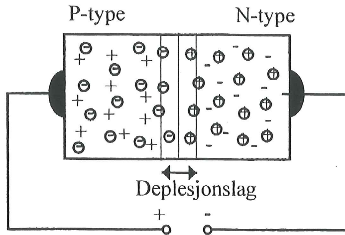
Fig. 3.9 Ytre spenning
