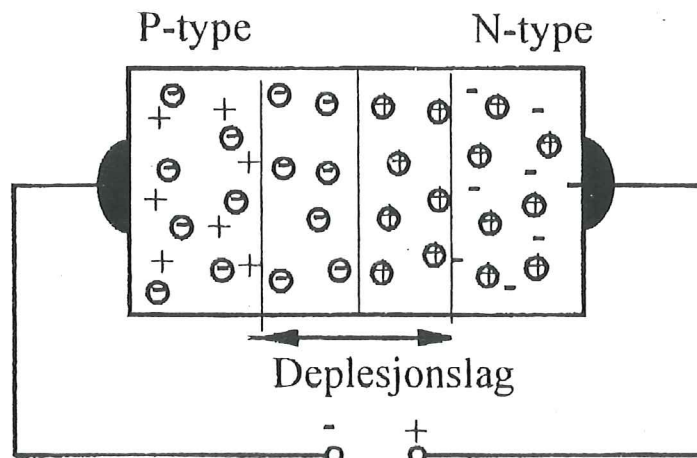
Fig. 3.8 Ytre spenning
