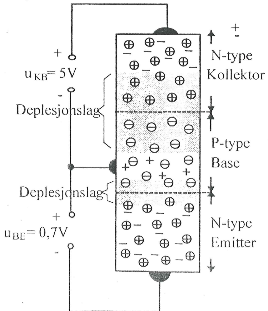
NPN-transistor
